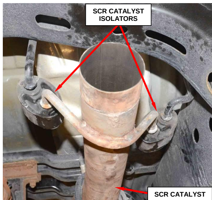
Figure 31 – SCR Catalyst Isolators
